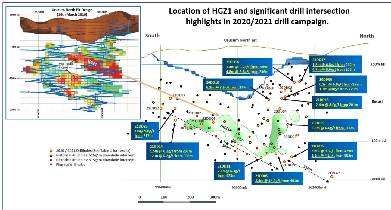
Figure 1: Location of HGZ1 and significant drill intersections highlights in the 2020 / 2021 drill campaign.
